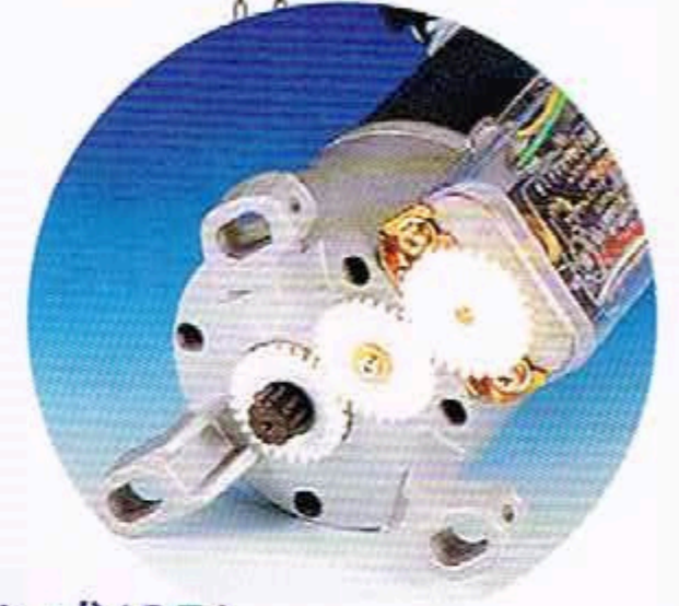
插心式(SP) (鍊條及齒輪已組裝完成) Slot-type(SP) (Chain & Gear Assembled)
